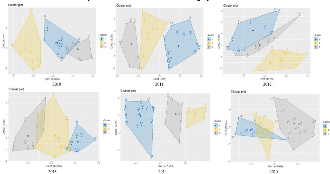
Figure 7. Clustering Results
