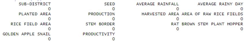
Figure 3 Missing Value
