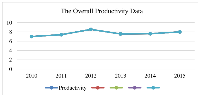
Figure 2 Explore Data
