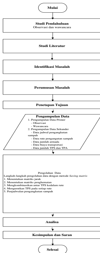
Gambar 1 Flowchart Penelitian
